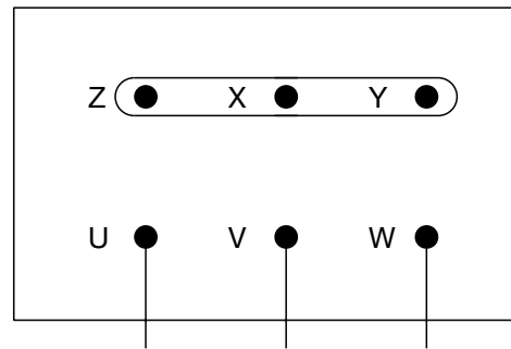
STAR ELECTRICAL CONNECTION
